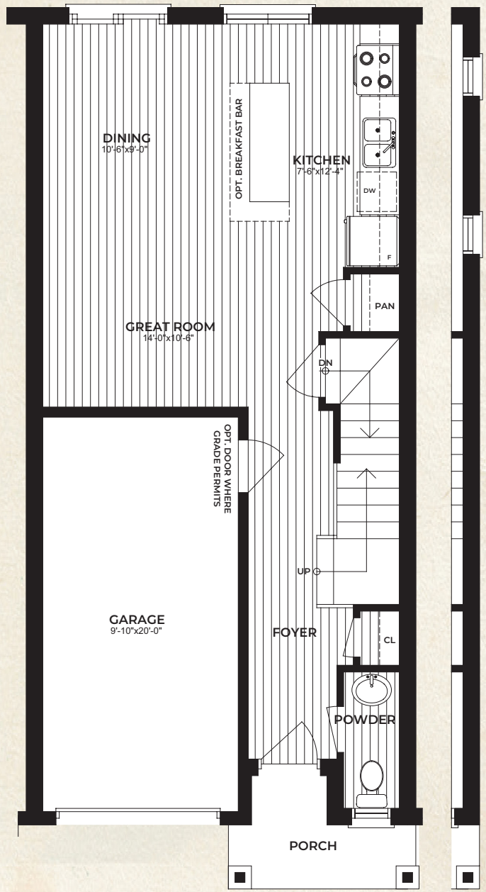
GROUND FLOOR OPTION 1B
