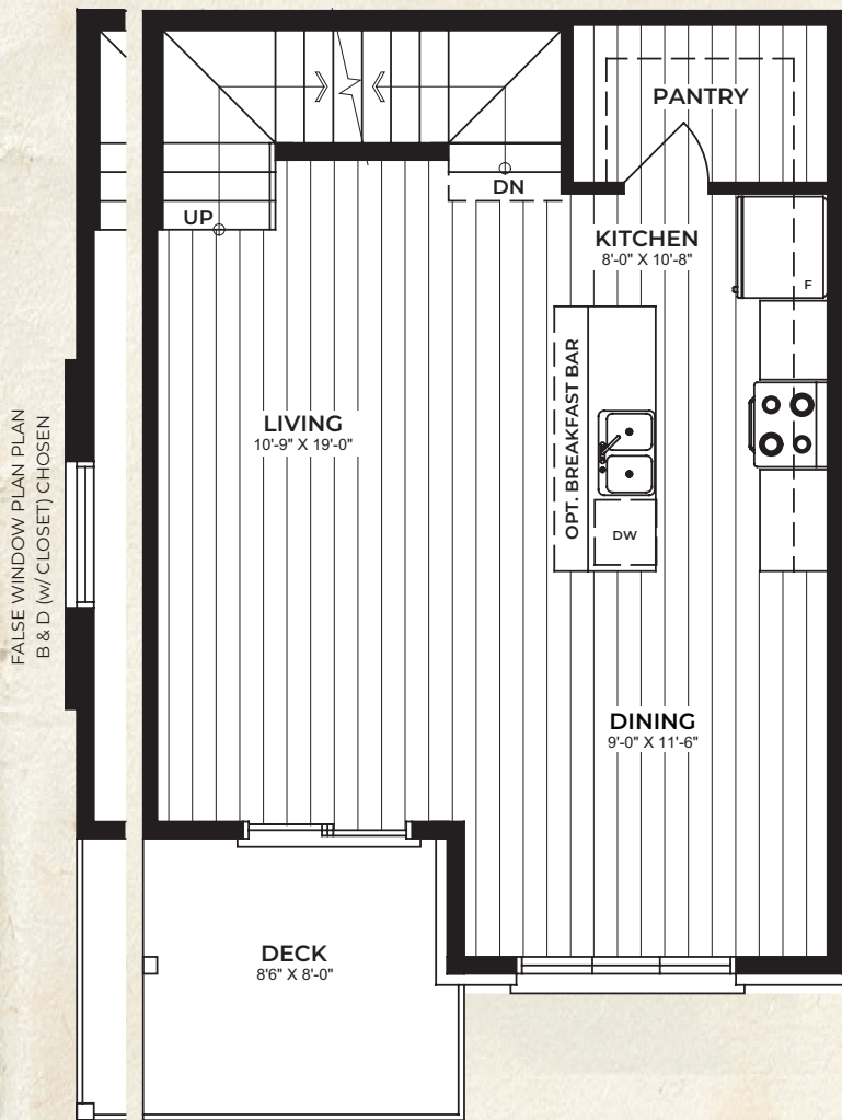
SECOND FLOOR OPT. A
