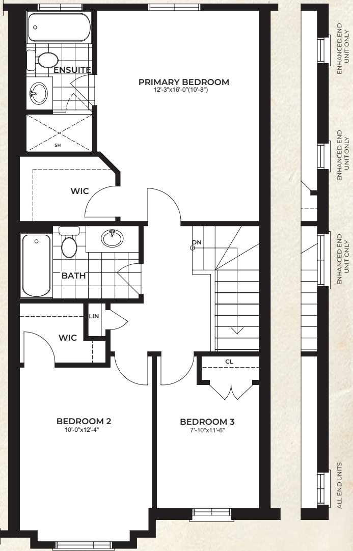
SECOND FLOOR OPTION 2B
