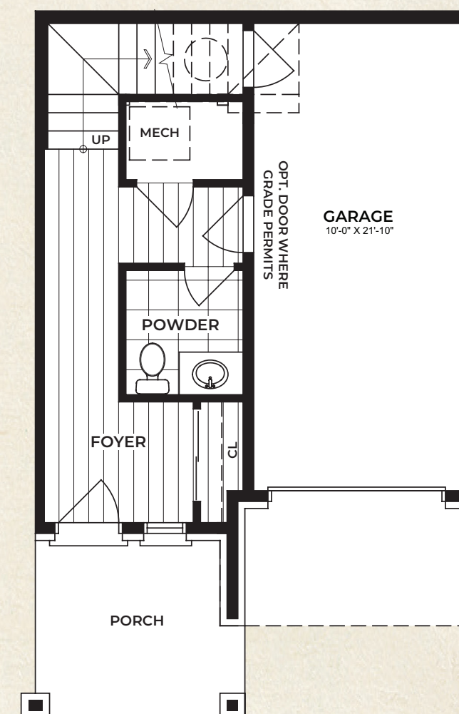
GROUND FLOOR OPT. D AVAILABLE WITH THIRD FLOOR OPTION B OR C ONLY
