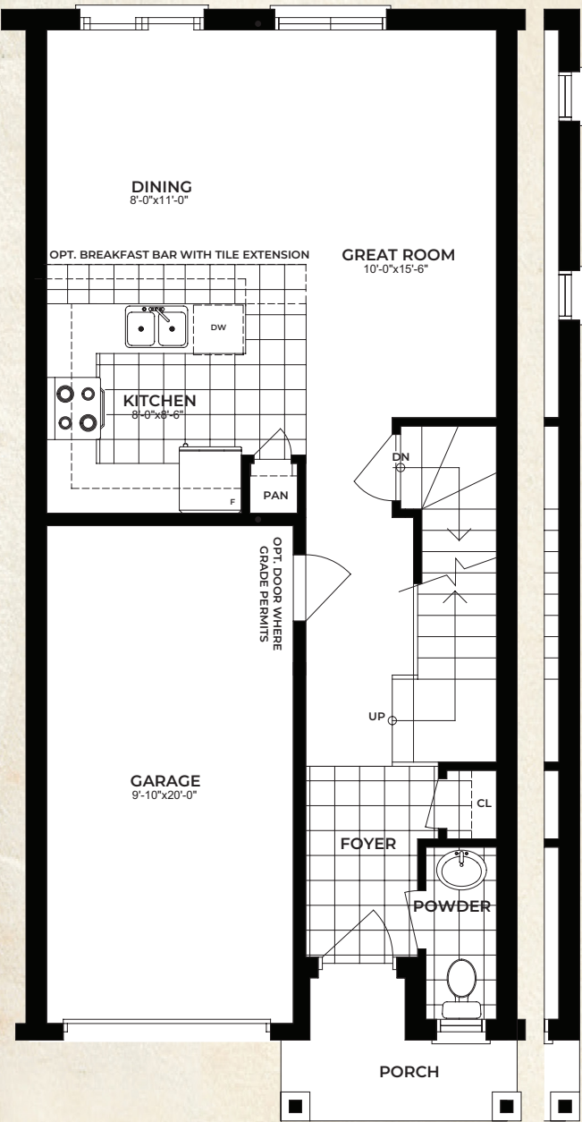
GROUND FLOOR OPTION 1A
