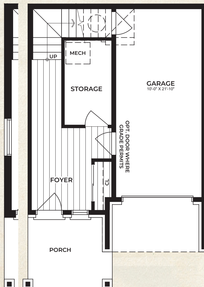
GROUND FLOOR OPT. A AVAILABLE WITH THIRD FLOOR OPTION B OR C ONLY
